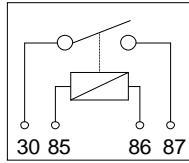
Normally open contacts
