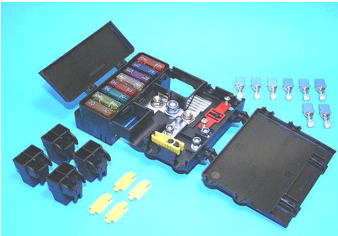
Battery mounted power distribution box. Page 20
