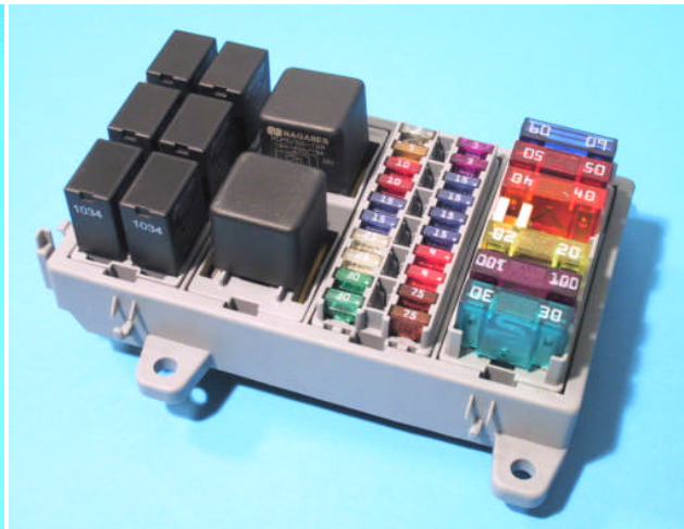
Modular fuse and relay system. Page 22
