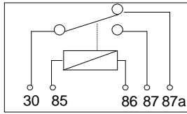
Change over contacts
